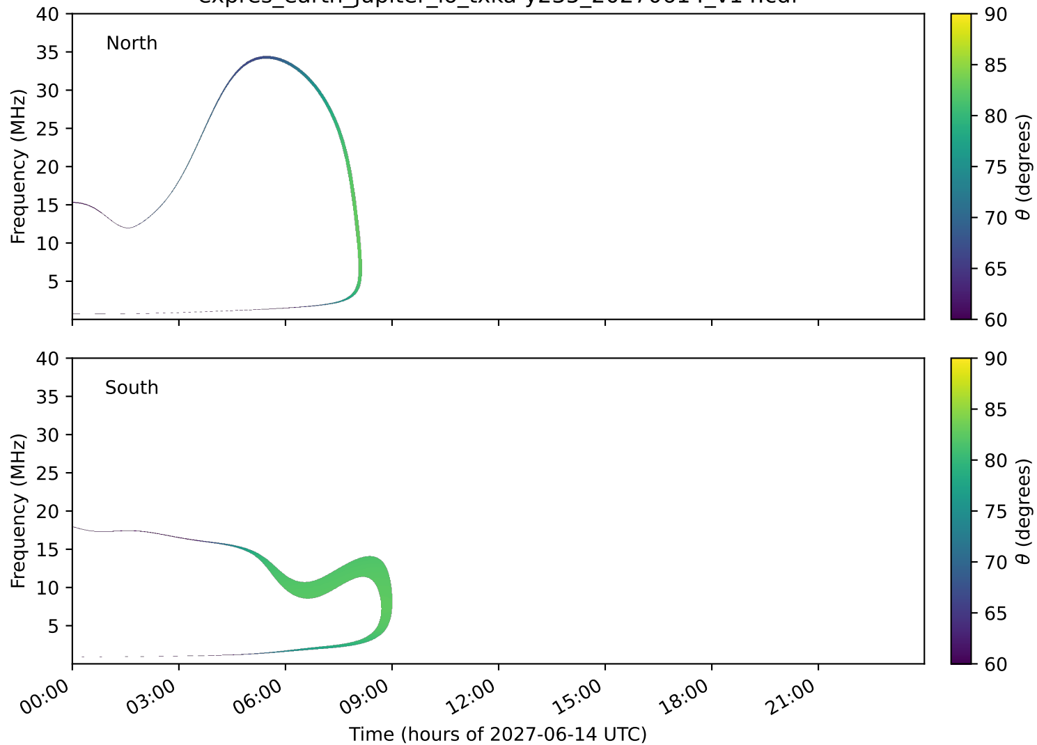
expres_earth_jupiter_io_txka-y235_20270614_v14.cdf
