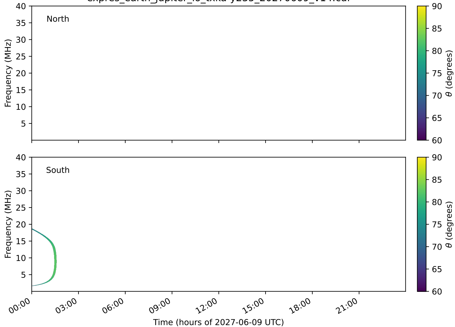
expres_earth_jupiter_io_txka-y235_20270609_v14.cdf
