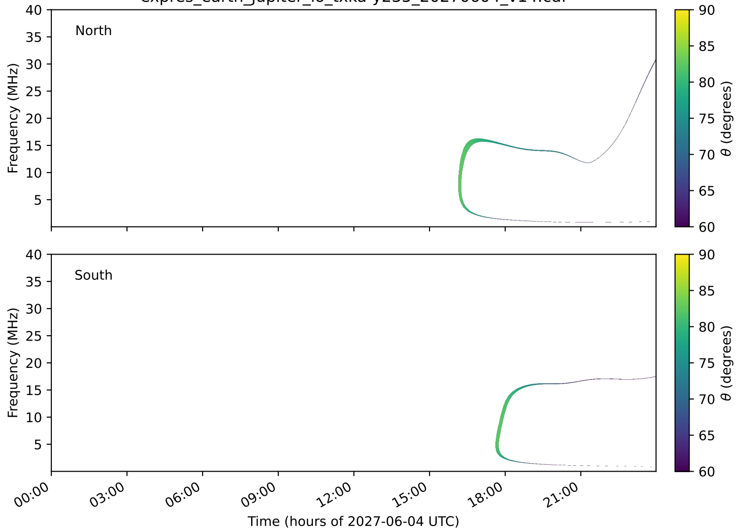
expres_earth_jupiter_io_txka-y235_20270604_v14.cdf
