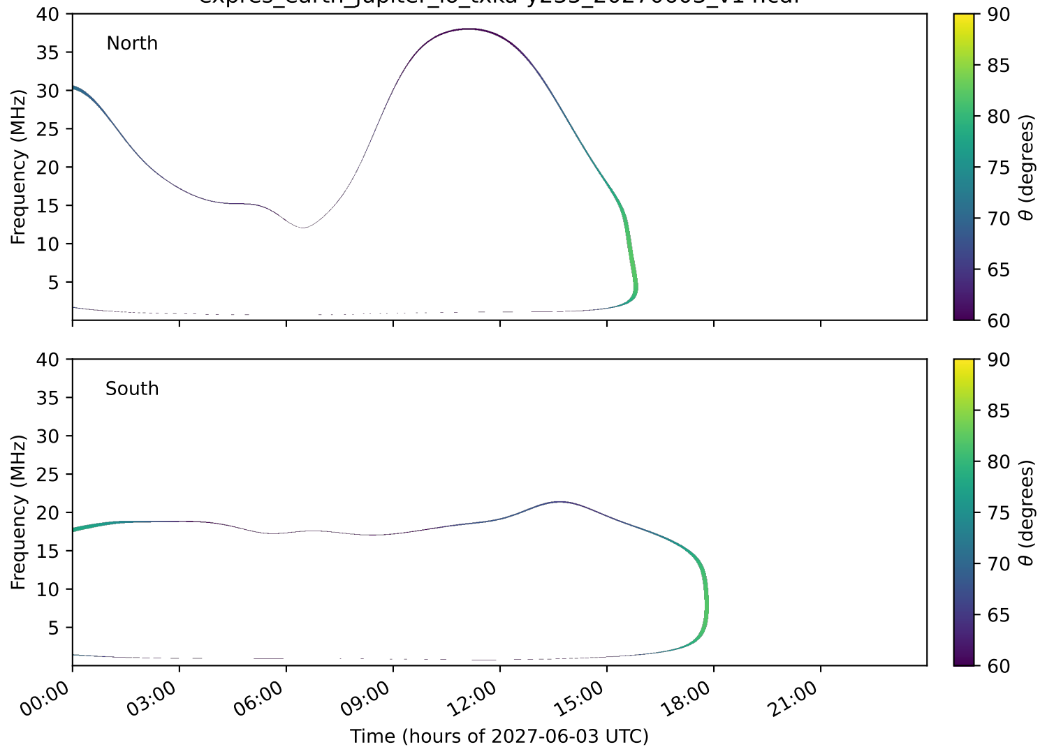
expres_earth_jupiter_io_txka-y235_20270603_v14.cdf
