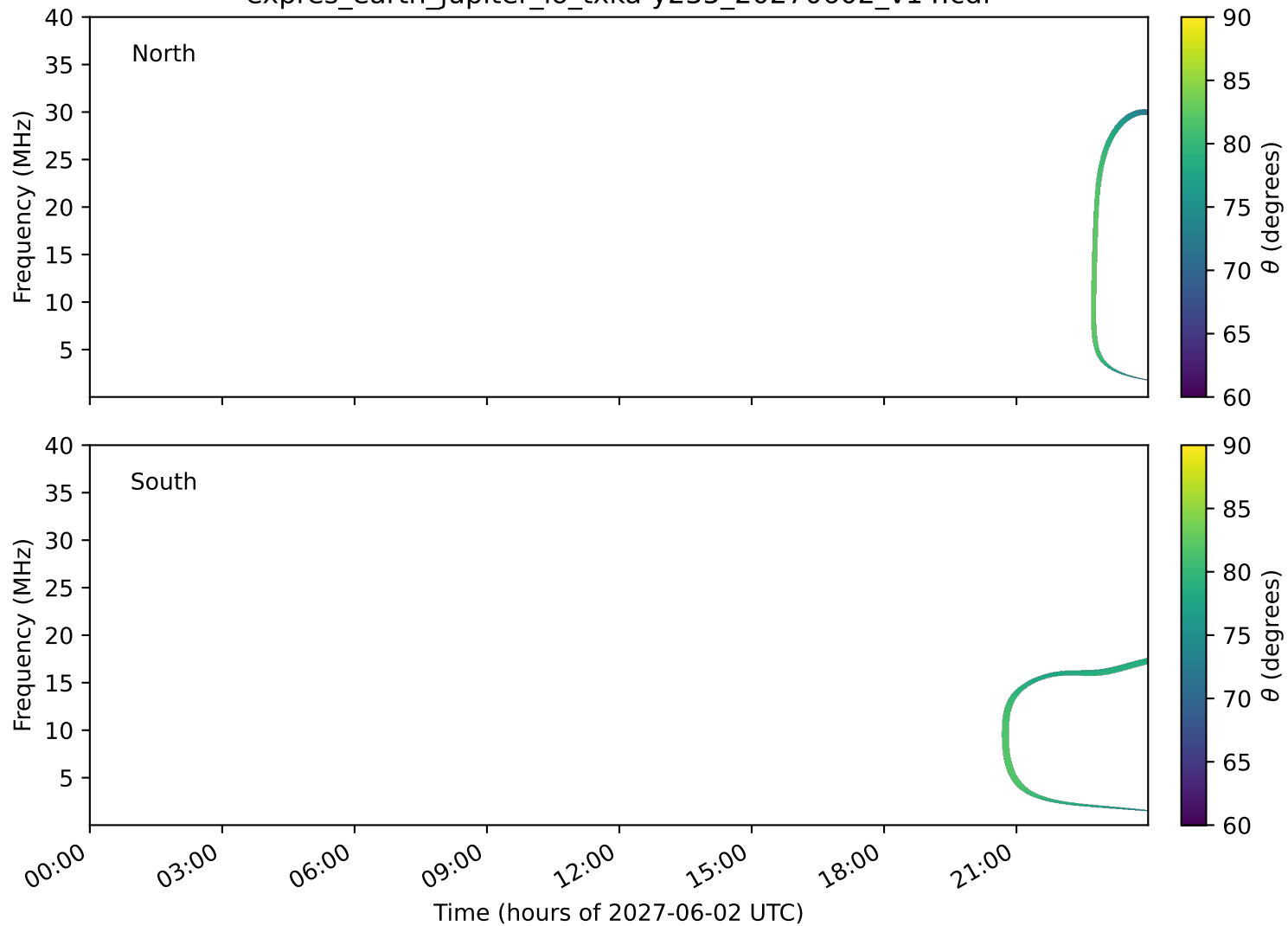
expres_earth_jupiter_io_txka-y235_20270602_v14.cdf
