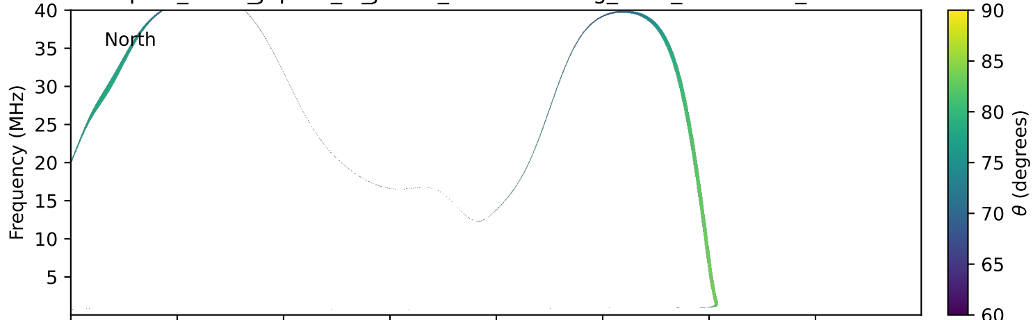
expres_earth_jupiter_io_jrm33_lossc-wid1deg_3kev_20270626_v11.cdf
