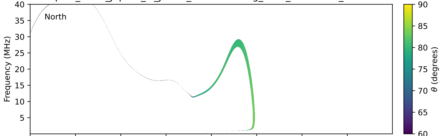
expres_earth_jupiter_io_jrm33_lossc-wid1deg_3kev_20270612_v11.cdf
