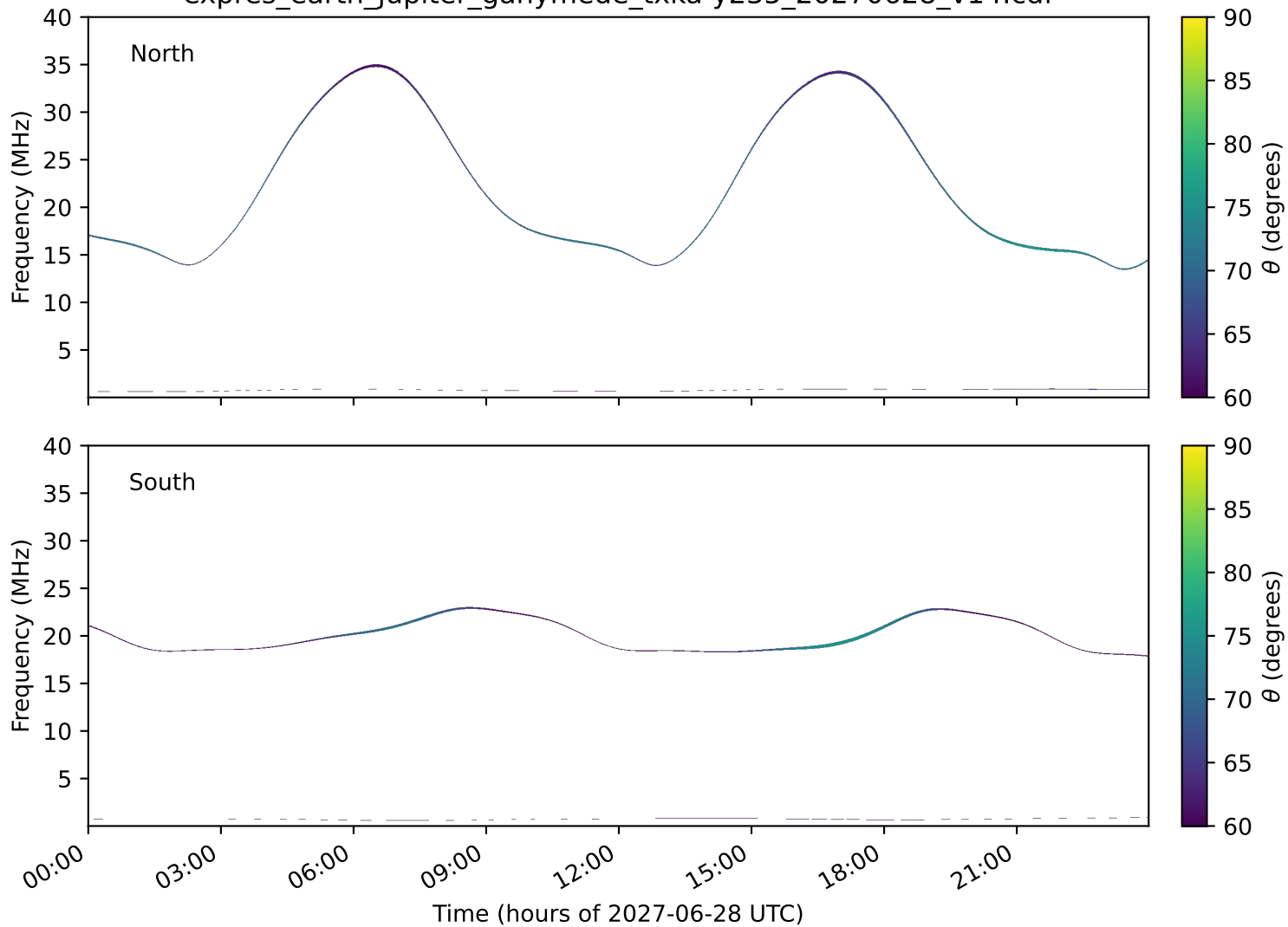
expres_earth_jupiter_ganymede_txka-y235_20270628_v14.cdf
