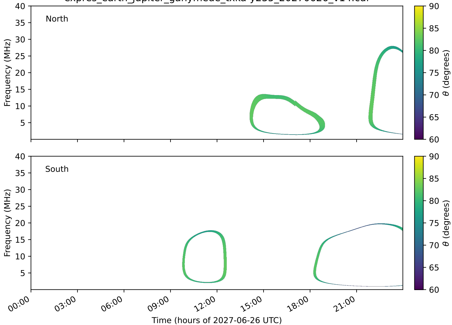
expres_earth_jupiter_ganymede_txka-y235_20270626_v14.cdf
