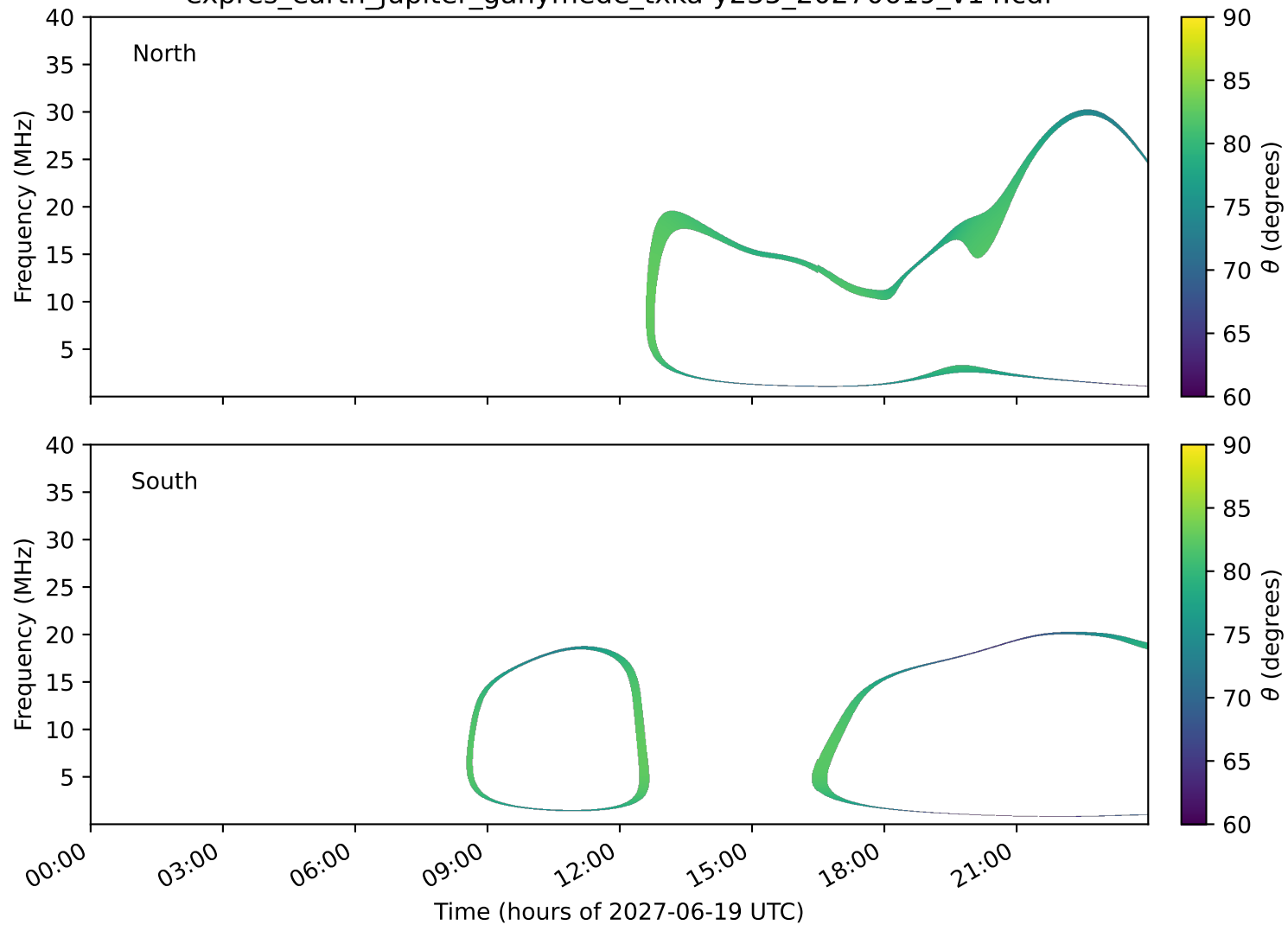
expres_earth_jupiter_ganymede_txka-y235_20270619_v14.cdf
