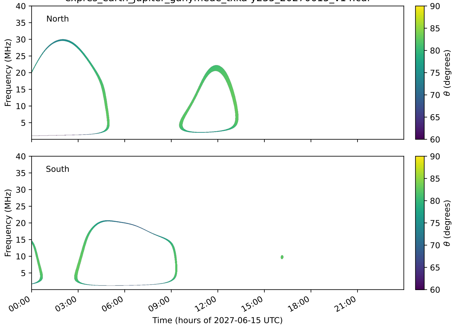
expres_earth_jupiter_ganymede_txka-y235_20270615_v14.cdf
