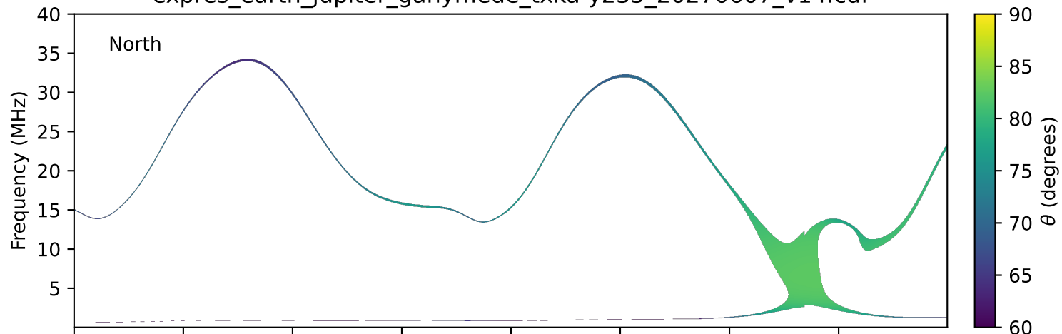
expres_earth_jupiter_ganymede_txka-y235_20270607_v14.cdf
