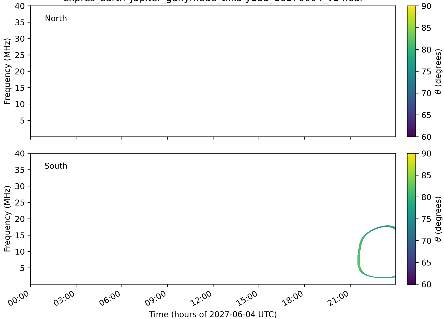
expres_earth_jupiter_ganymede_txka-y235_20270604_v14.cdf
