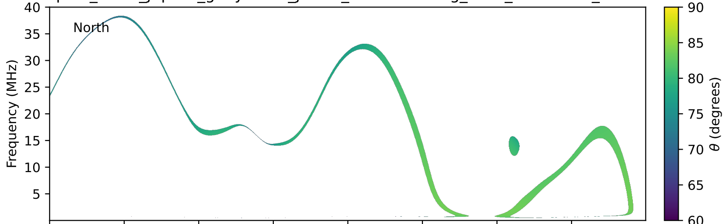
expres_earth_jupiter_ganymede_jrm33_lossc-wid1deg_3kev_20270622_v11.cdf
