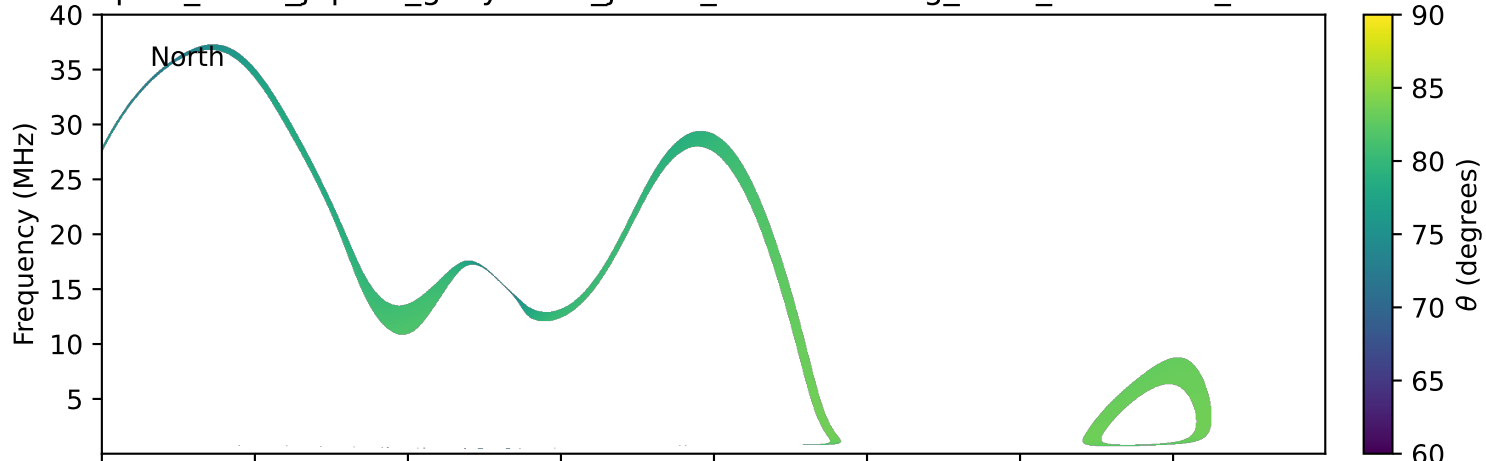
expres_earth_jupiter_ganymede_jrm33_lossc-wid1deg_3kev_20270615_v11.cdf
