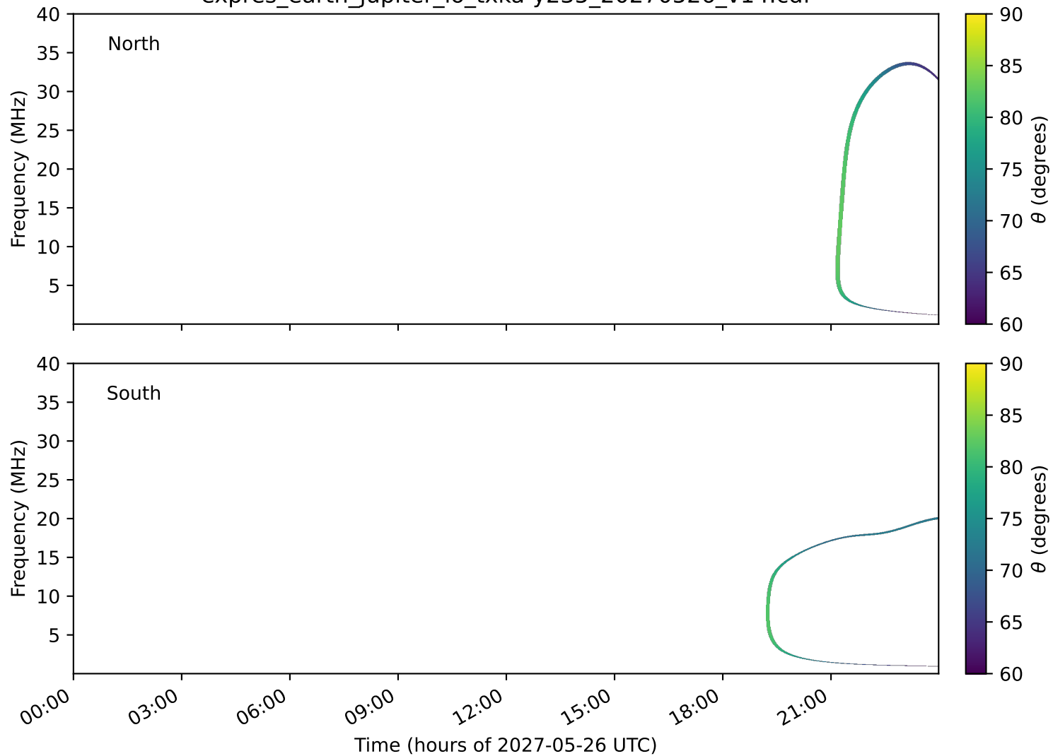
expres_earth_jupiter_io_txka-y235_20270526_v14.cdf
