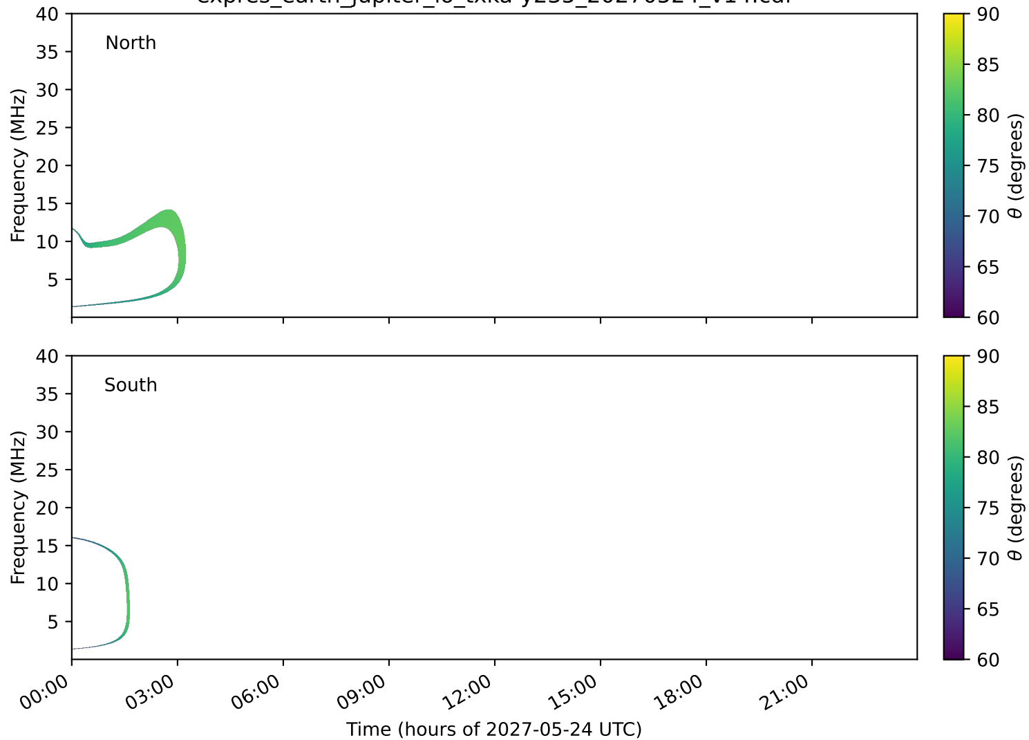
expres_earth_jupiter_io_txka-y235_20270524_v14.cdf
