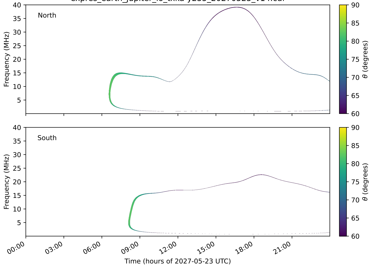
expres_earth_jupiter_io_txka-y235_20270523_v14.cdf
