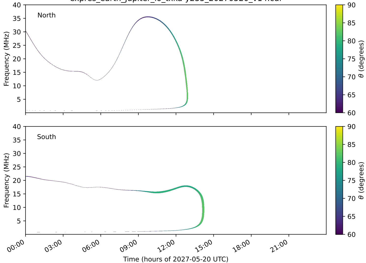
expres_earth_jupiter_io_txka-y235_20270520_v14.cdf
