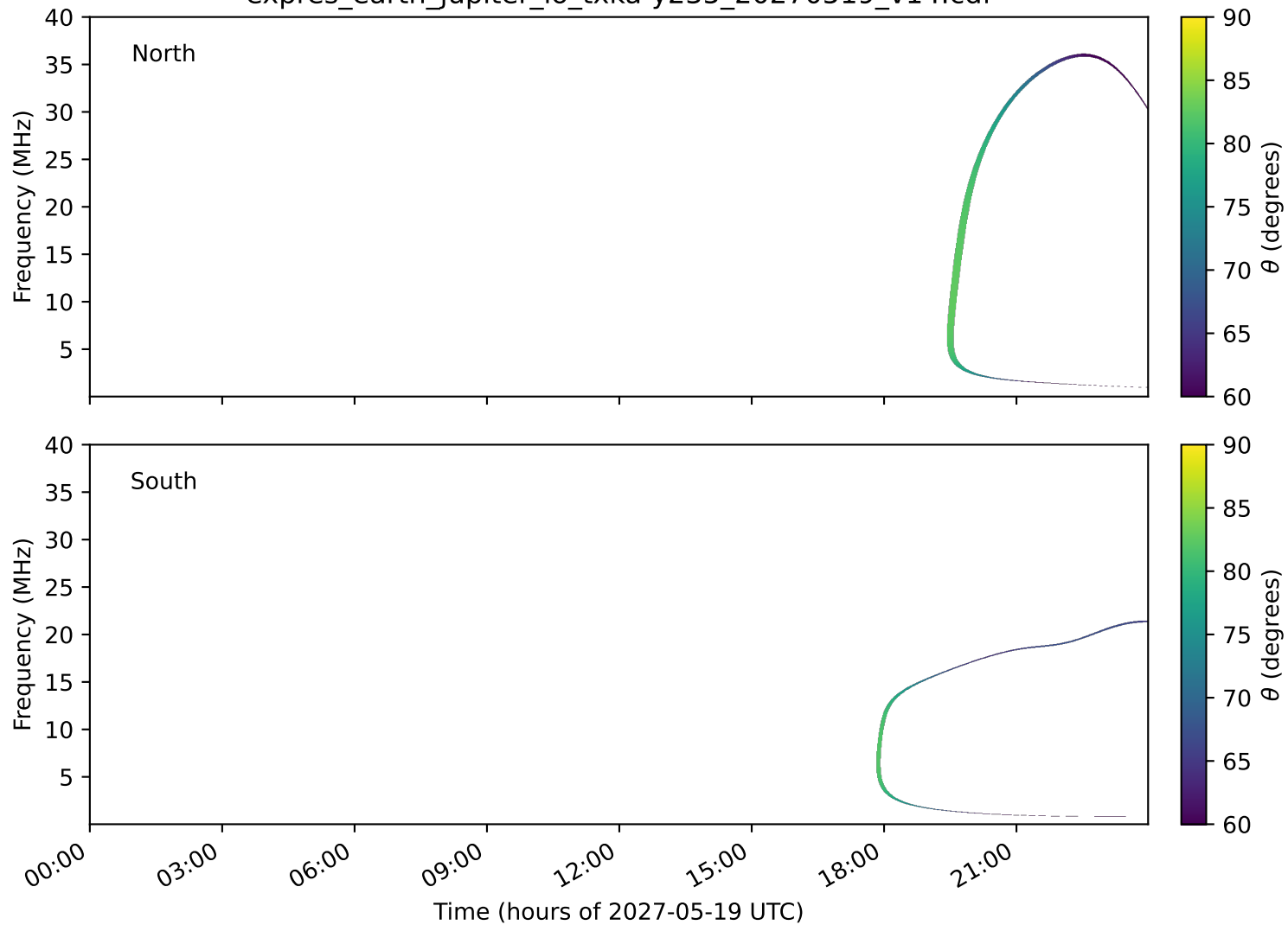
expres_earth_jupiter_io_txka-y235_20270519_v14.cdf
