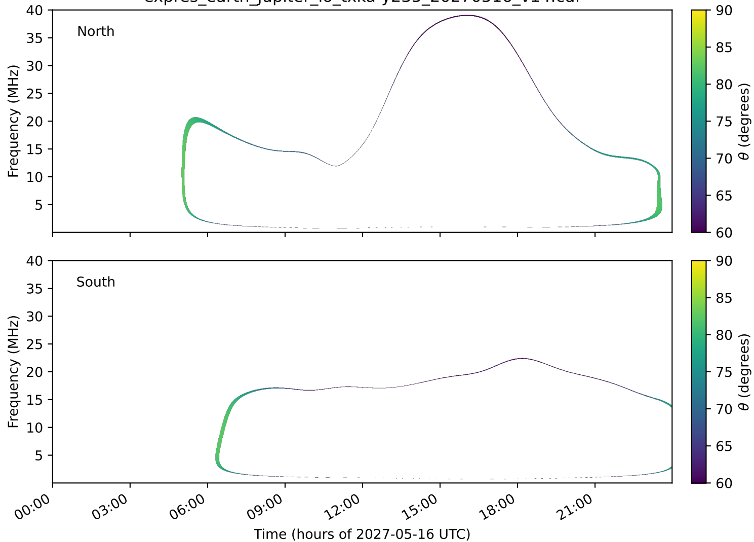
expres_earth_jupiter_io_txka-y235_20270516_v14.cdf
