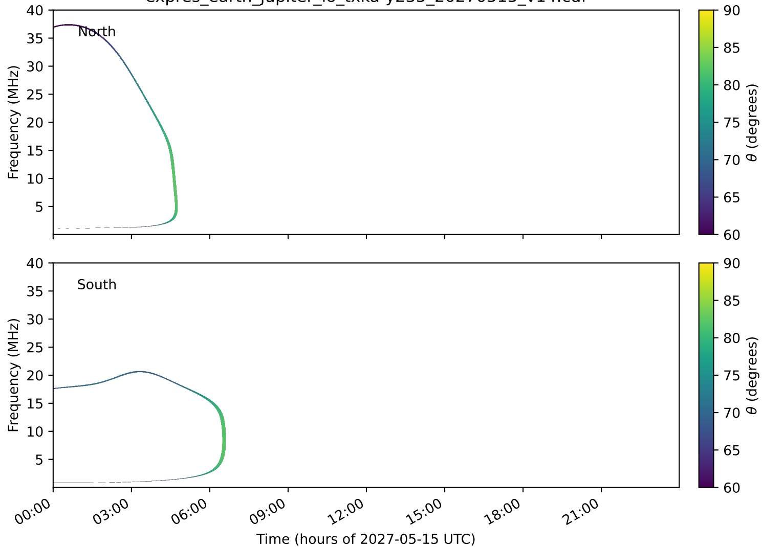
expres_earth_jupiter_io_txka-y235_20270515_v14.cdf
