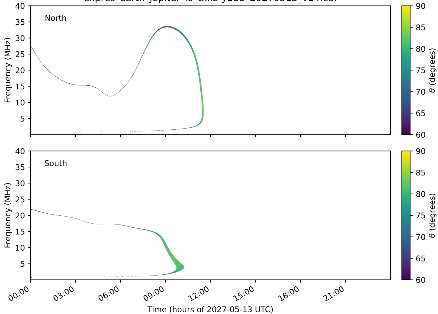
expres_earth_jupiter_io_txka-y235_20270513_v14.cdf
