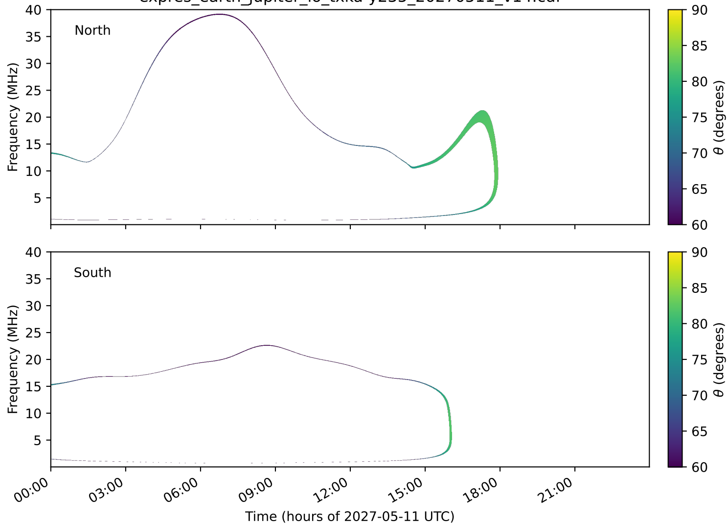
expres_earth_jupiter_io_txka-y235_20270511_v14.cdf
