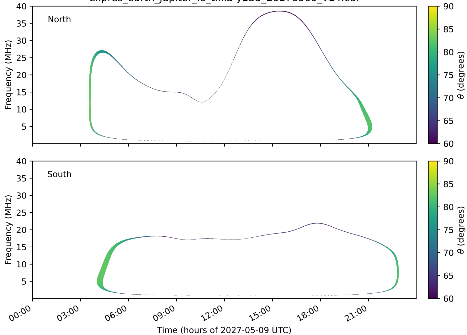
expres_earth_jupiter_io_txka-y235_20270509_v14.cdf
