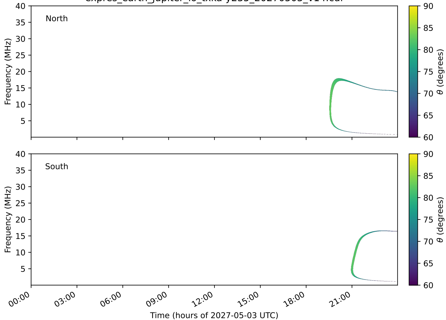
expres_earth_jupiter_io_txka-y235_20270503_v14.cdf
