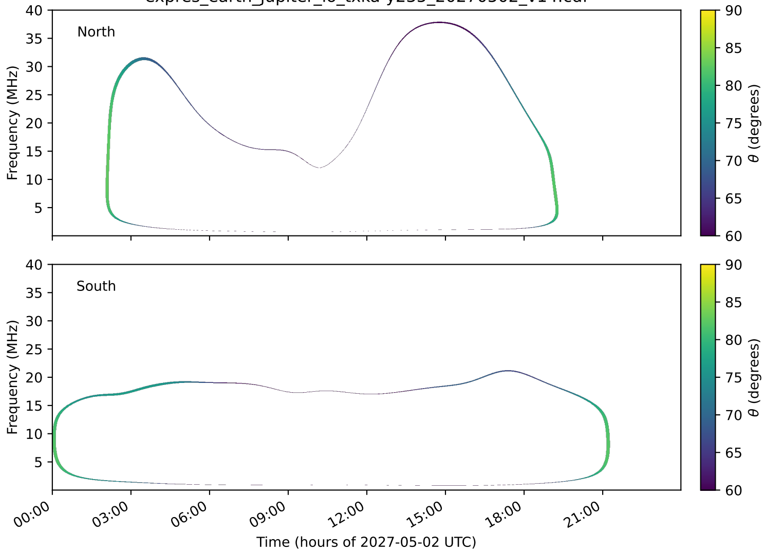
expres_earth_jupiter_io_txka-y235_20270502_v14.cdf
