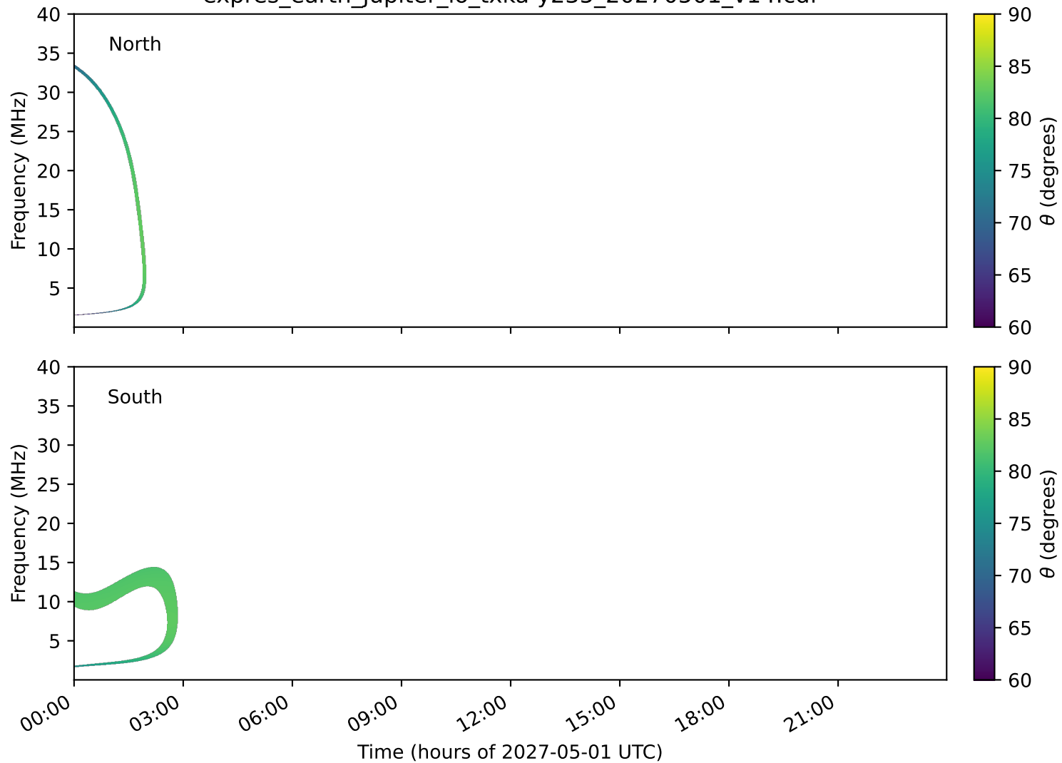
expres_earth_jupiter_io_txka-y235_20270501_v14.cdf
