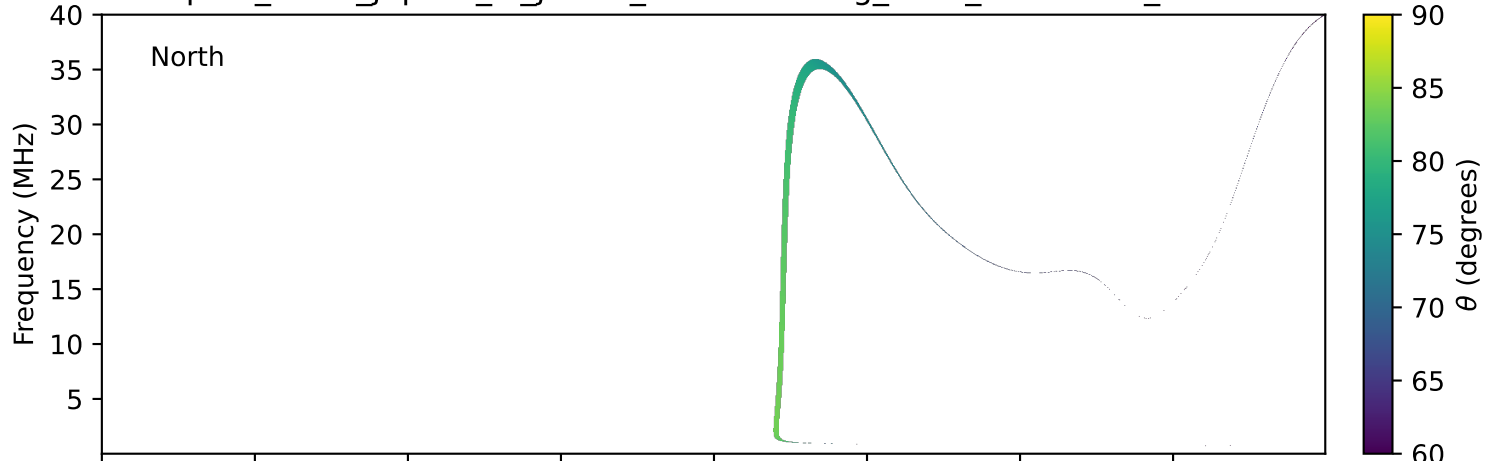
expres_earth_jupiter_io_jrm33_lossc-wid1deg_3kev_20270521_v11.cdf
