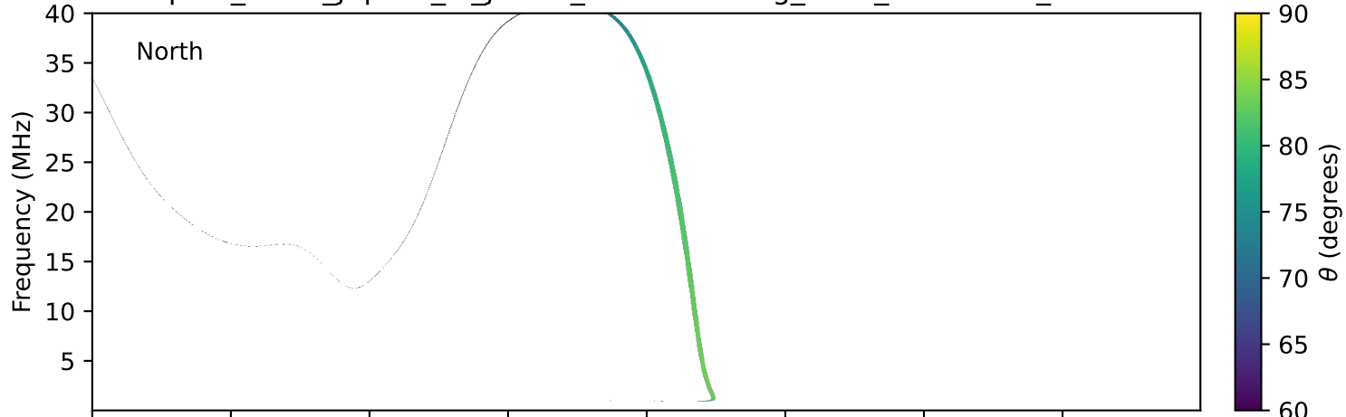
expres_earth_jupiter_io_jrm33_lossc-wid1deg_3kev_20270520_v11.cdf
