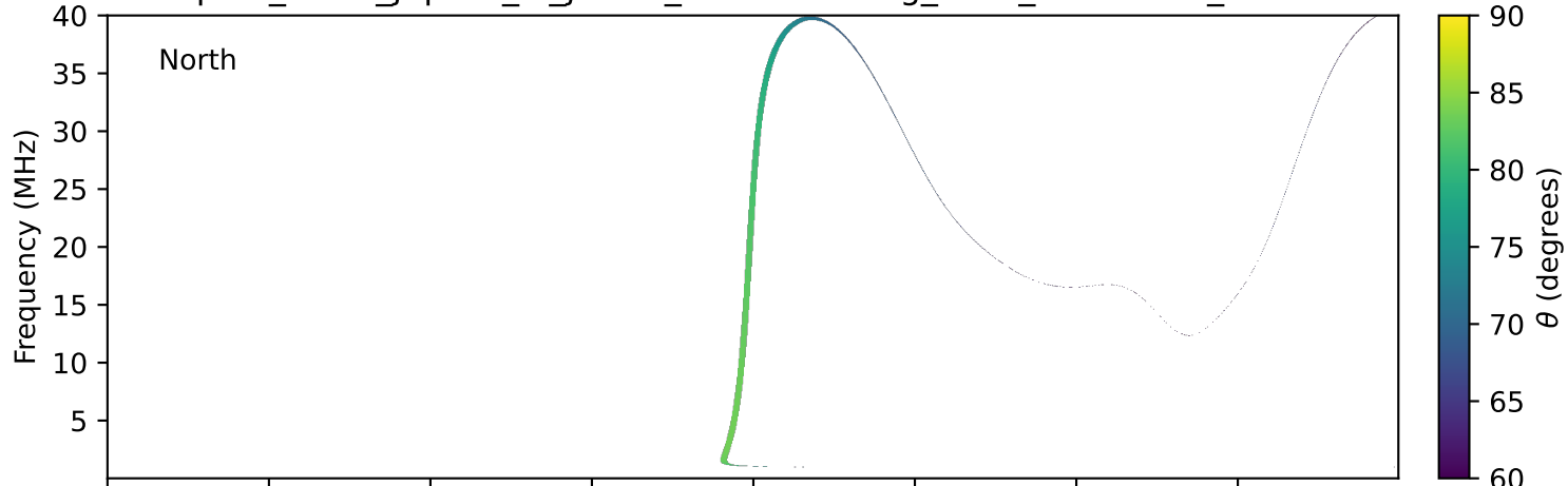
expres_earth_jupiter_io_jrm33_lossc-wid1deg_3kev_20270514_v11.cdf
