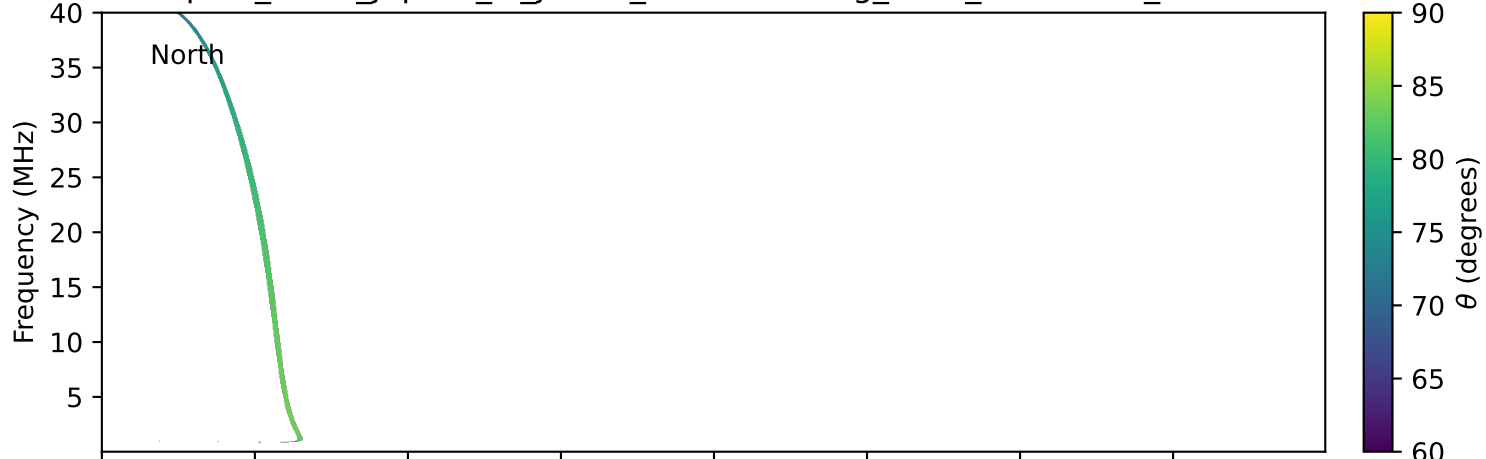
expres_earth_jupiter_io_jrm33_lossc-wid1deg_3kev_20270508_v11.cdf
