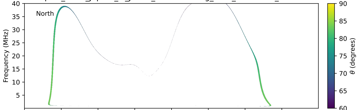
expres_earth_jupiter_io_jrm33_lossc-wid1deg_3kev_20270502_v11.cdf
