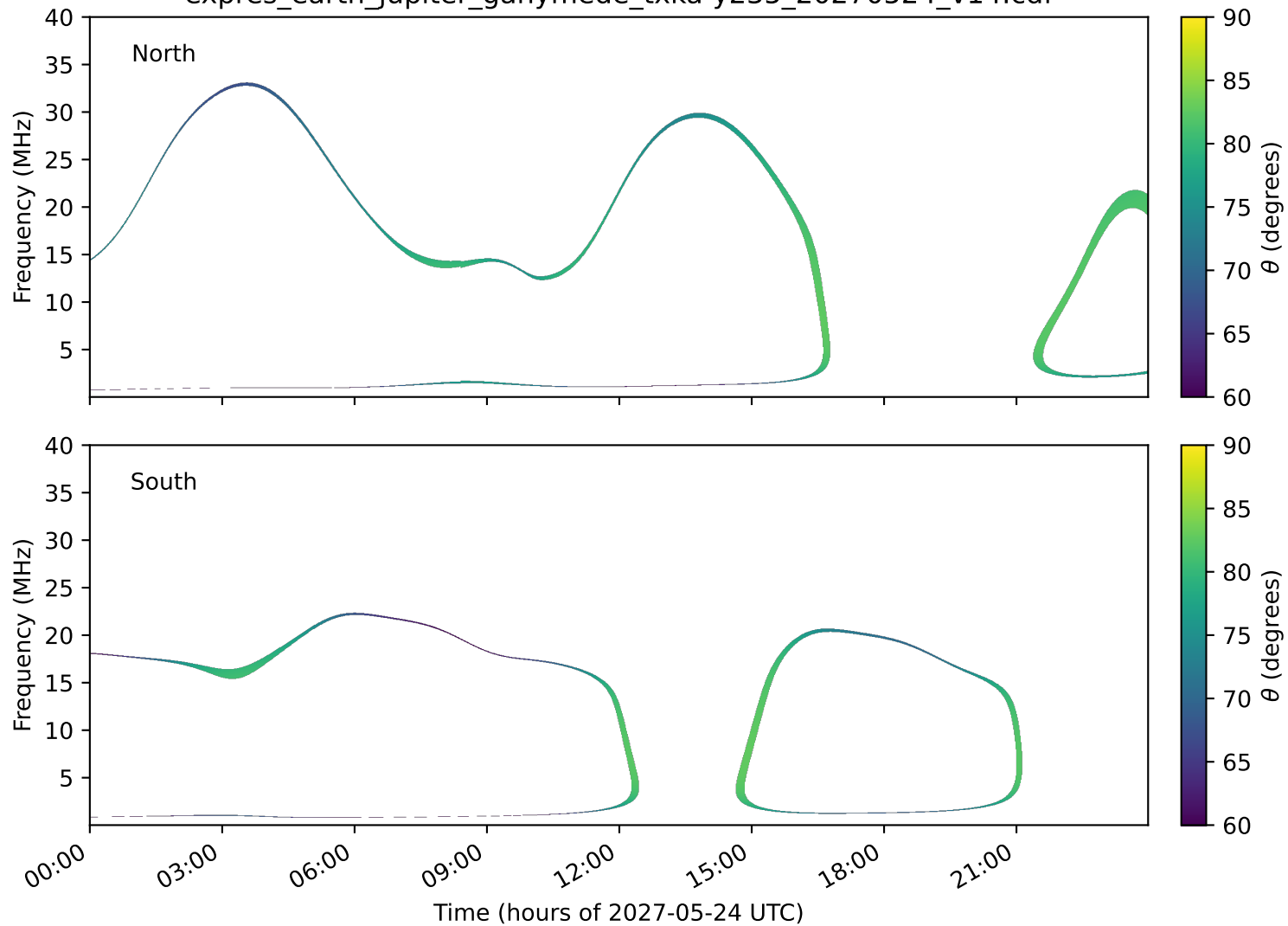
expres_earth_jupiter_ganymede_txka-y235_20270524_v14.cdf
