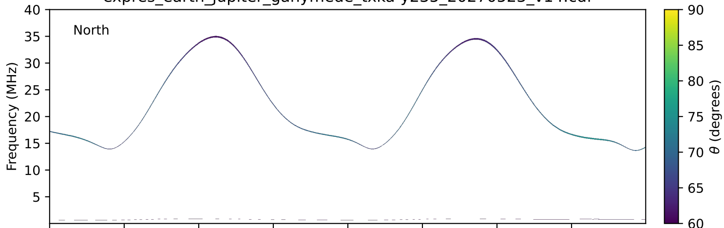
expres_earth_jupiter_ganymede_txka-y235_20270523_v14.cdf
