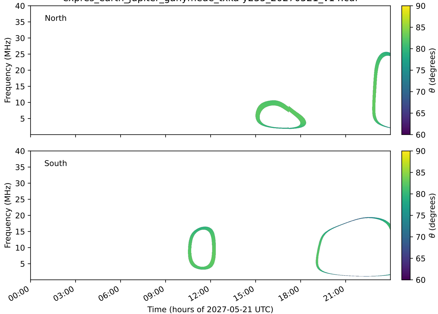
expres_earth_jupiter_ganymede_txka-y235_20270521_v14.cdf
