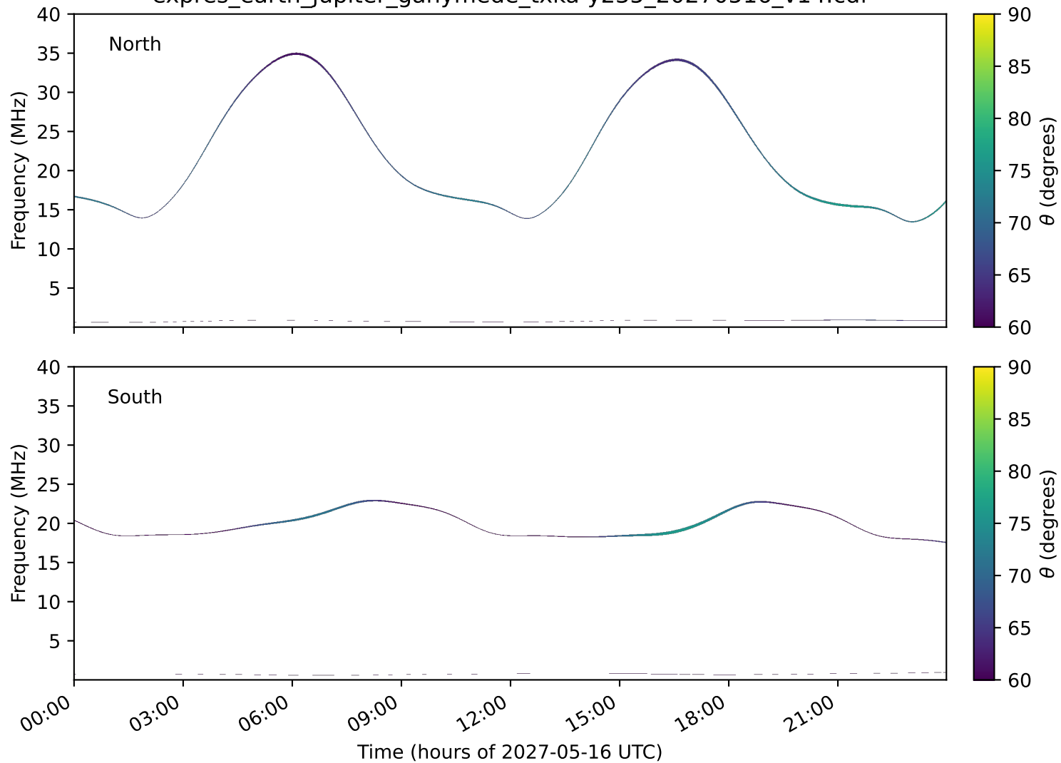
expres_earth_jupiter_ganymede_txka-y235_20270516_v14.cdf
