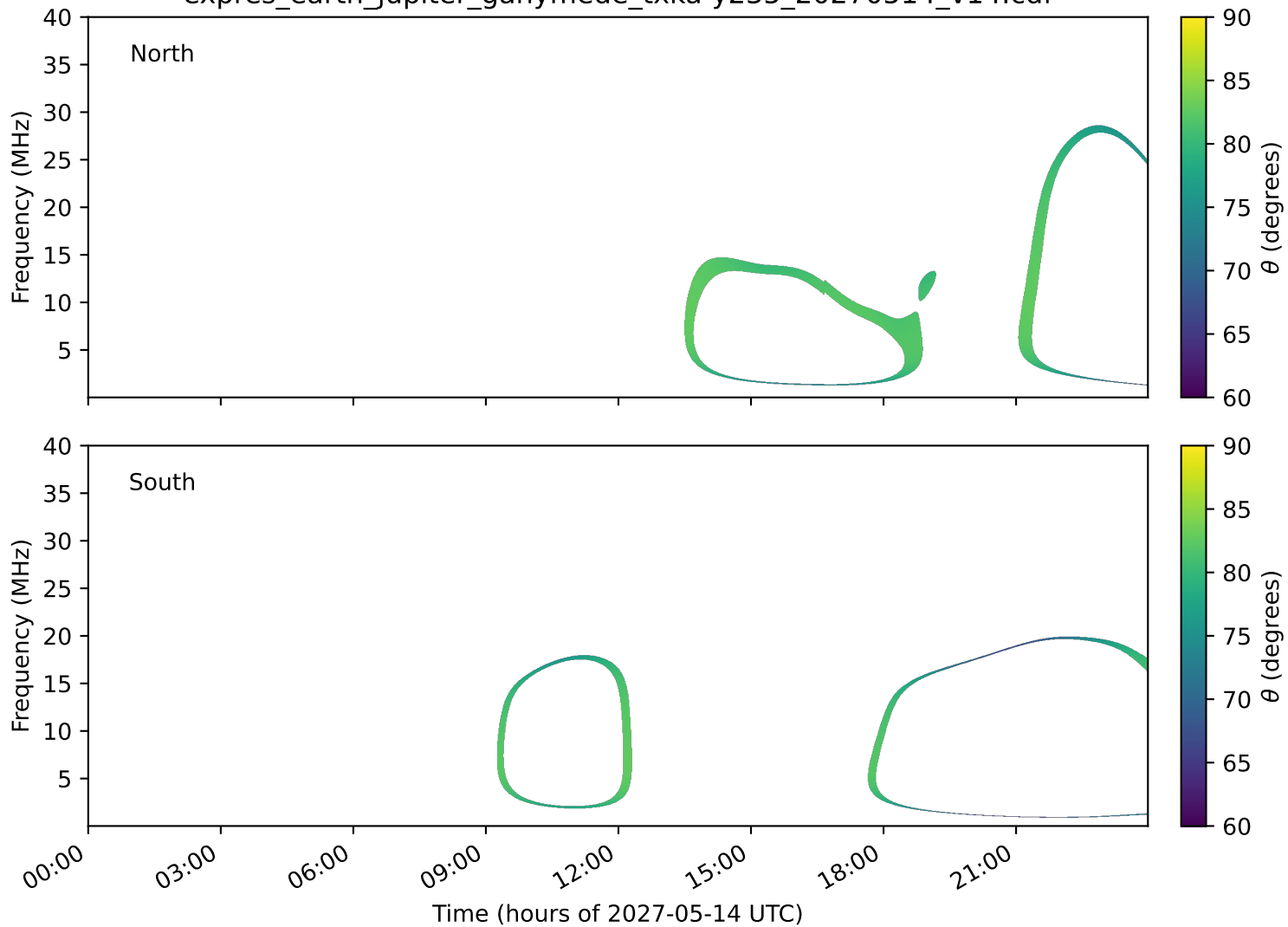
expres_earth_jupiter_ganymede_txka-y235_20270514_v14.cdf
