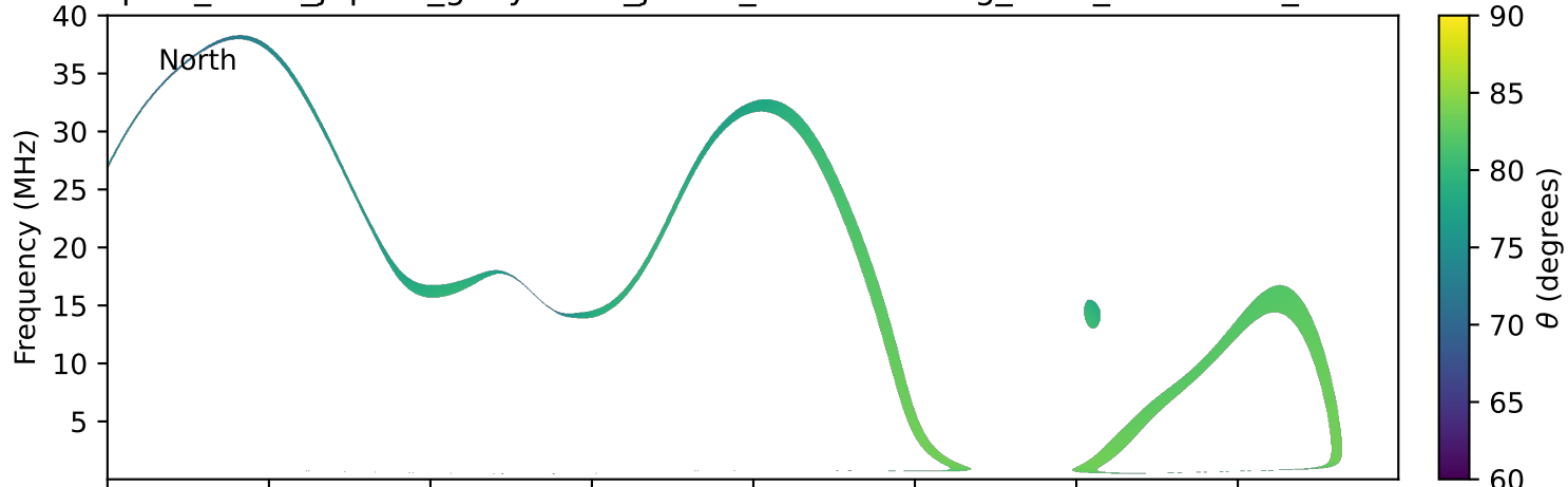
expres_earth_jupiter_ganymede_jrm33_lossc-wid1deg_3kev_20270510_v11.cdf
