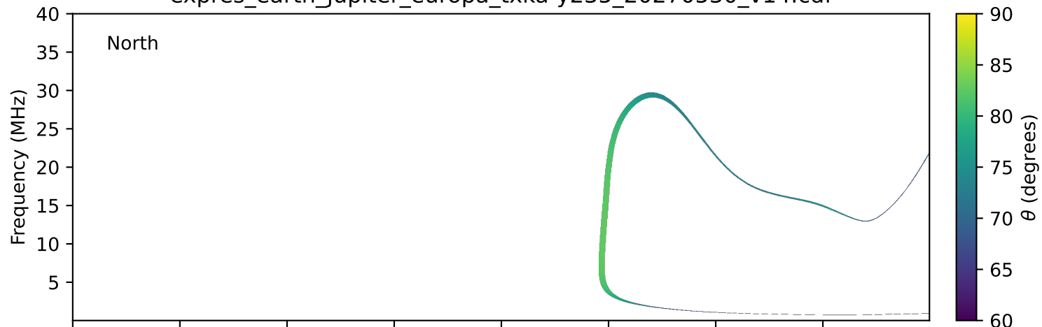
expres_earth_jupiter_europa_txka-y235_20270530_v14.cdf
