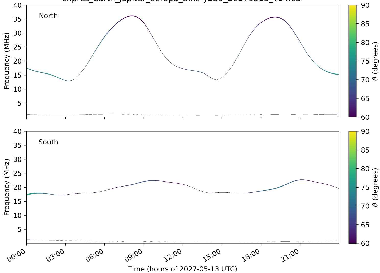
expres_earth_jupiter_europa_txka-y235_20270513_v14.cdf
