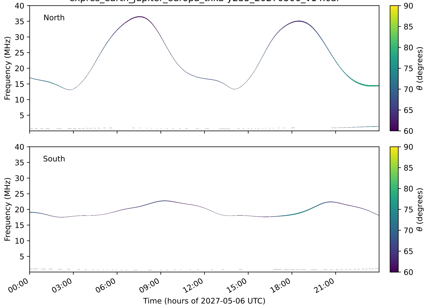
expres_earth_jupiter_europa_txka-y235_20270506_v14.cdf
