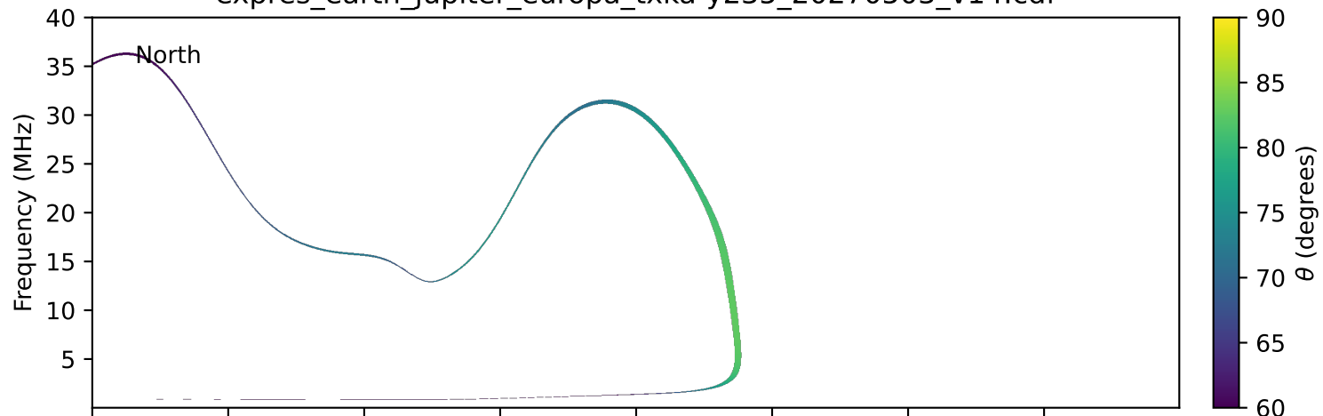
expres_earth_jupiter_europa_txka-y235_20270503_v14.cdf
