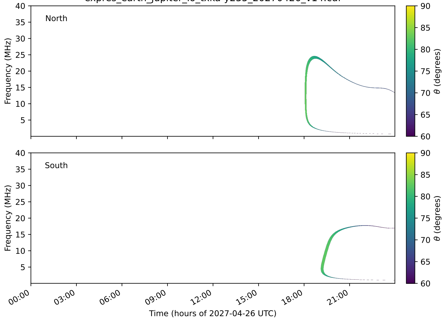
expres_earth_jupiter_io_txka-y235_20270426_v14.cdf
