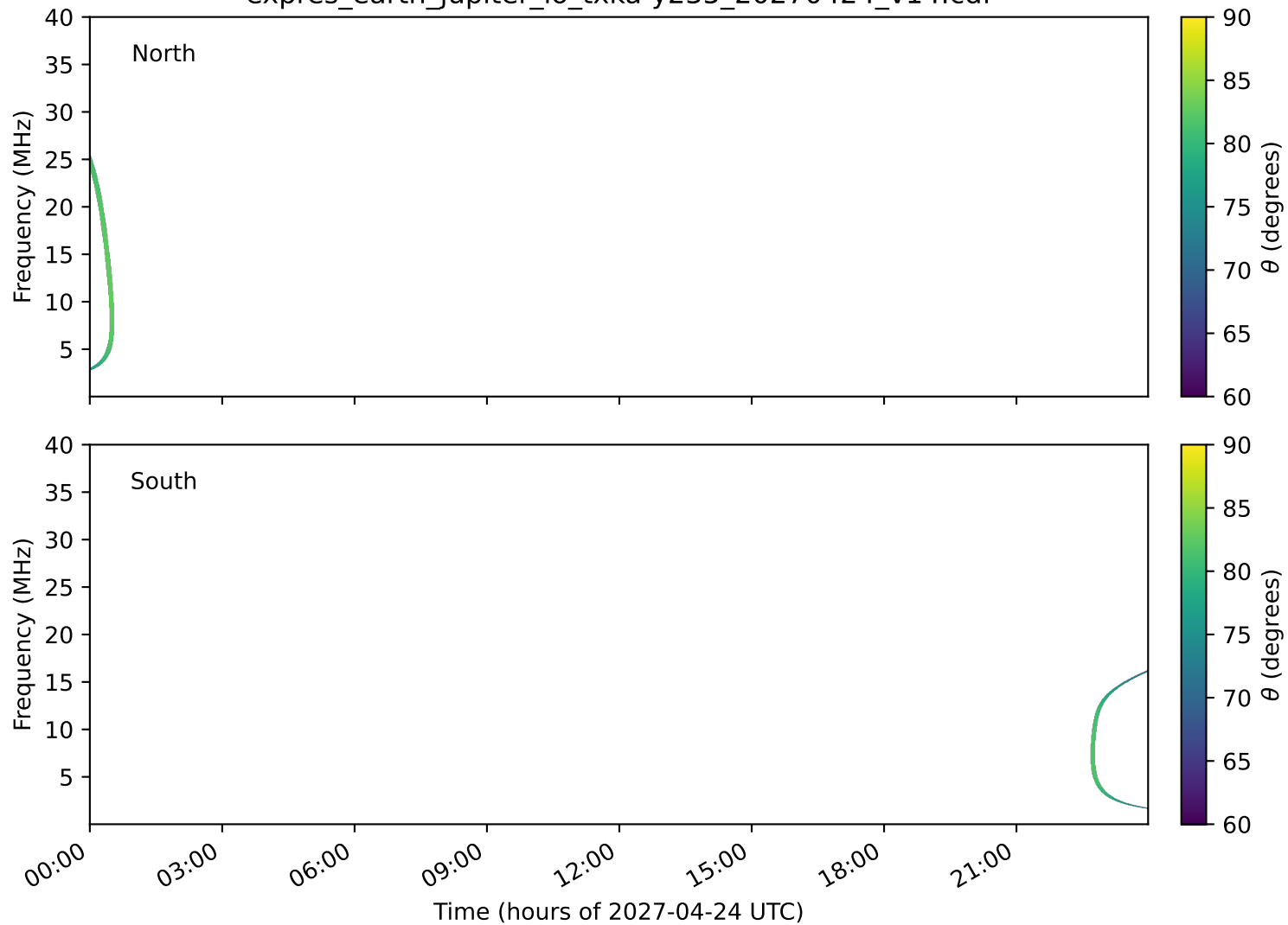
expres_earth_jupiter_io_txka-y235_20270424_v14.cdf
