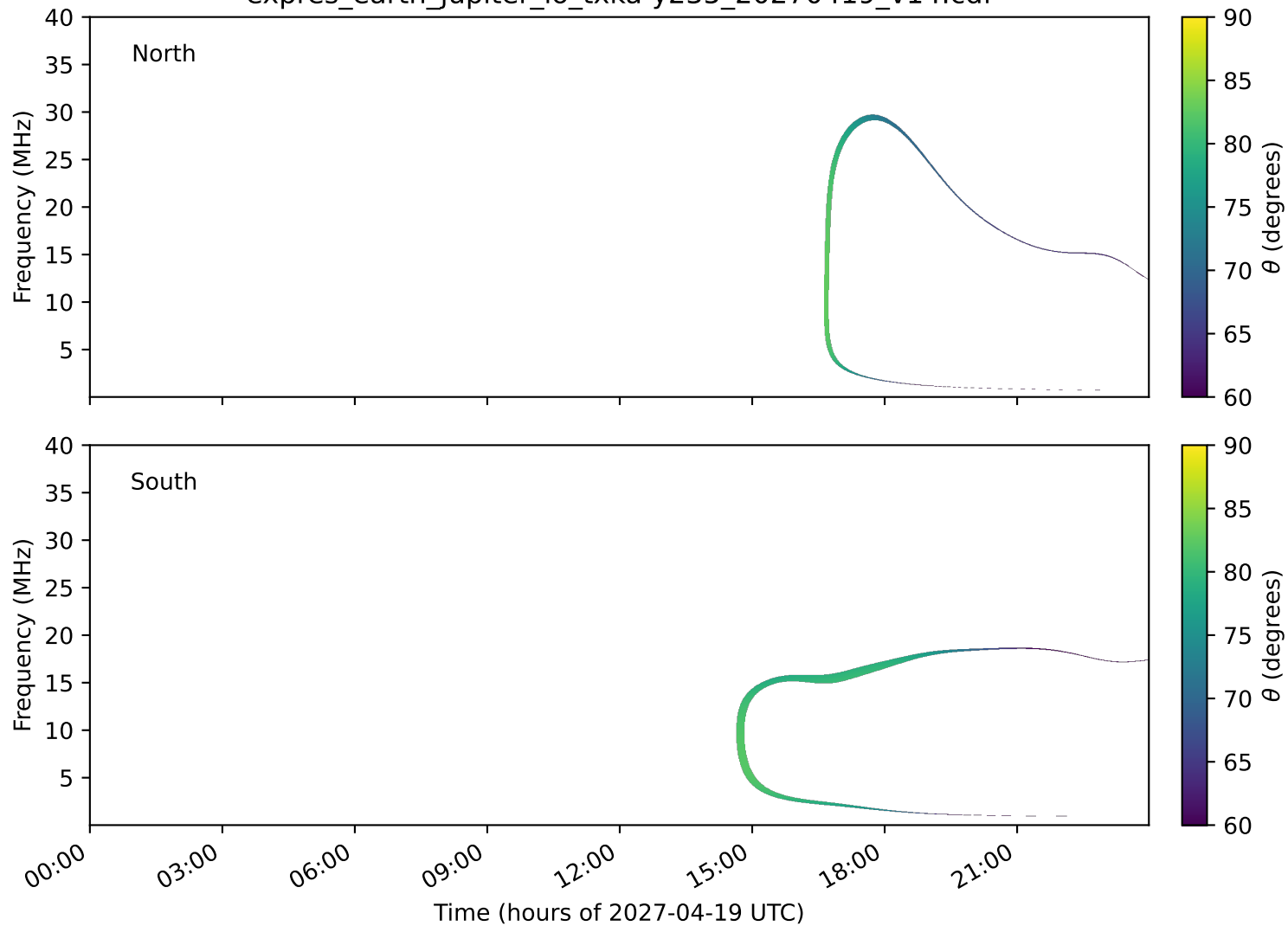
expres_earth_jupiter_io_txka-y235_20270419_v14.cdf
