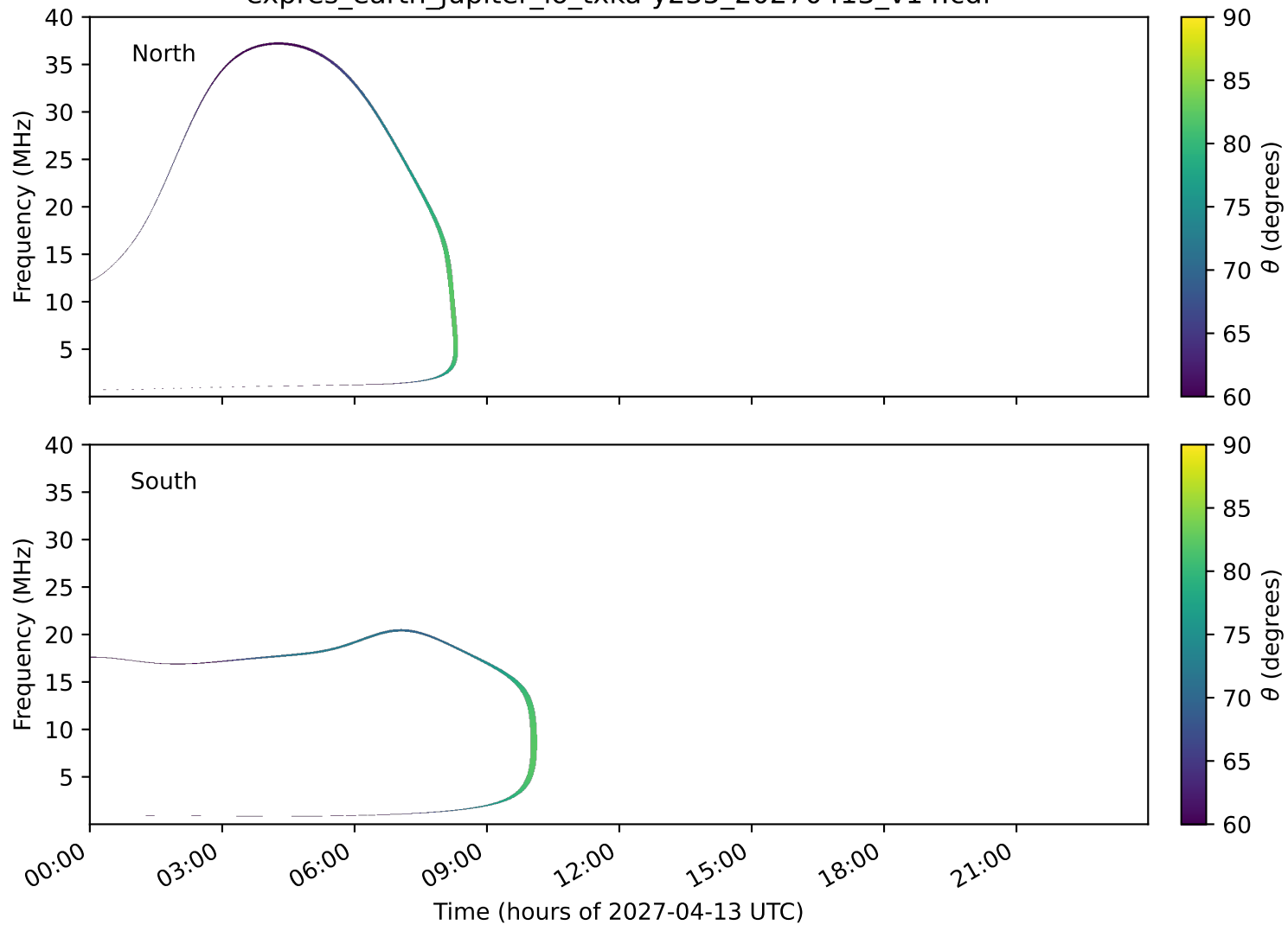
expres_earth_jupiter_io_txka-y235_20270413_v14.cdf
