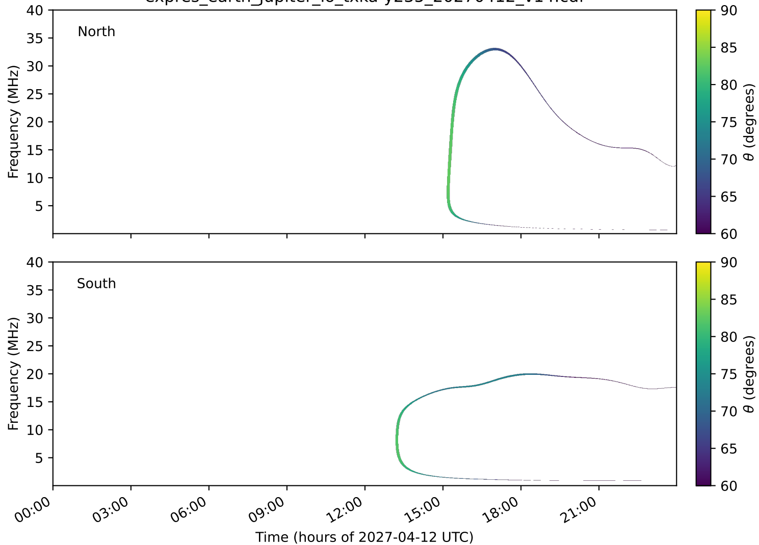
expres_earth_jupiter_io_txka-y235_20270412_v14.cdf
