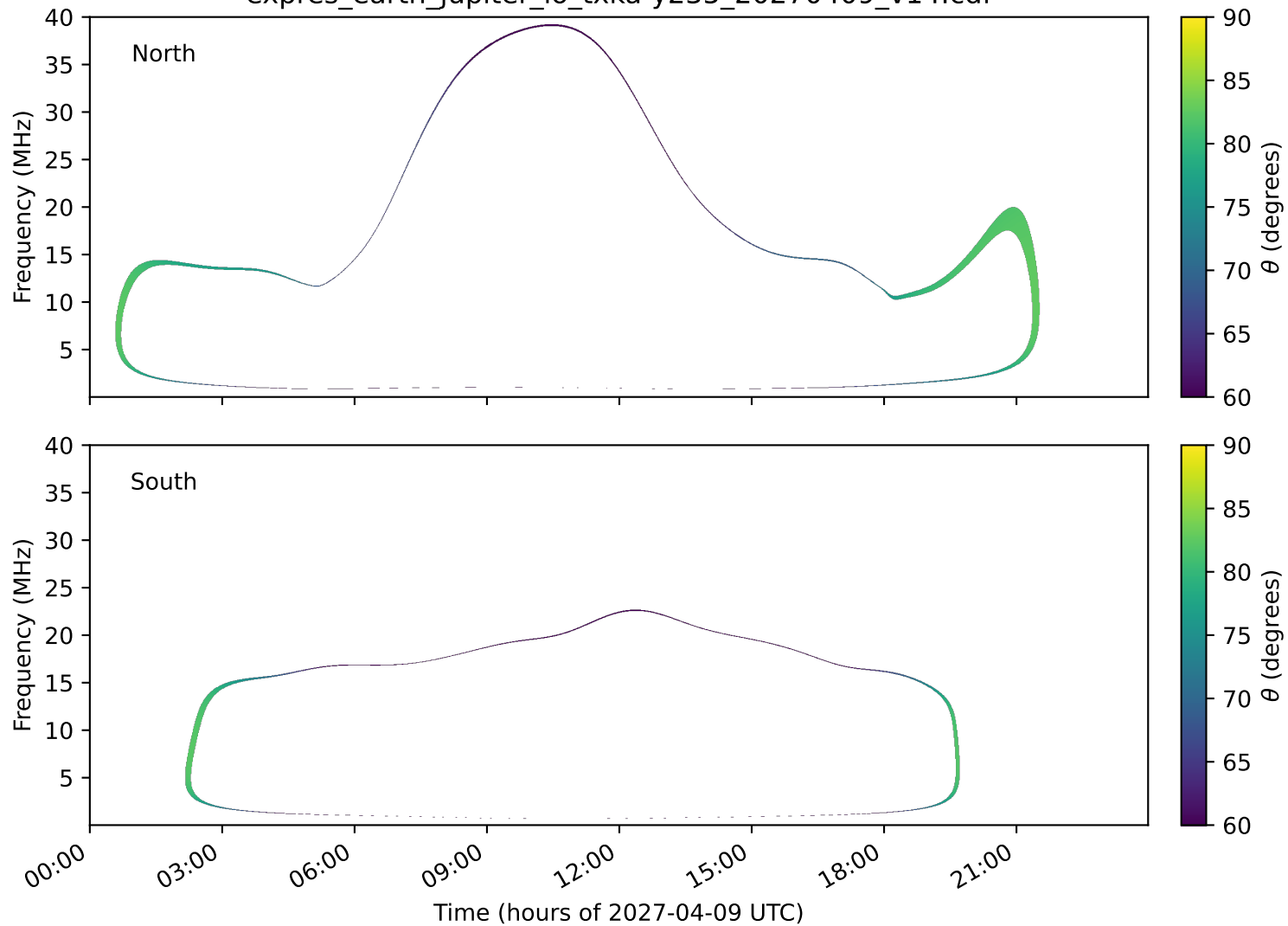
expres_earth_jupiter_io_txka-y235_20270409_v14.cdf
