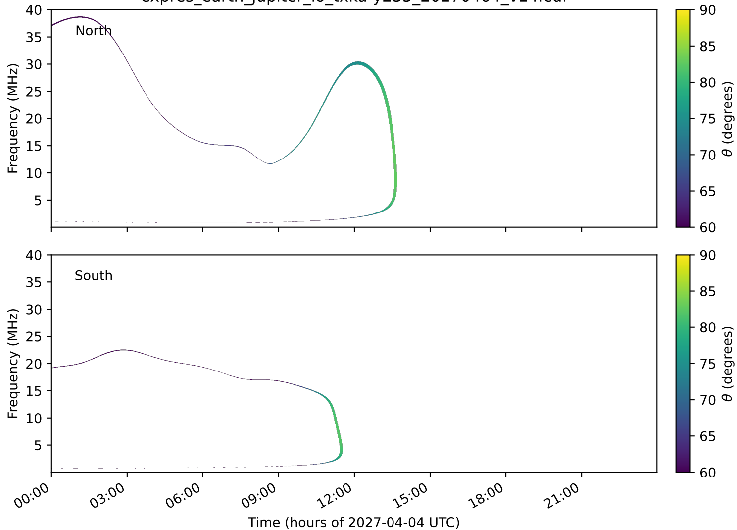
expres_earth_jupiter_io_txka-y235_20270404_v14.cdf
